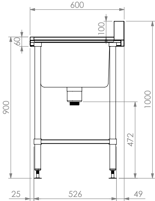
*600mm DEEP MODULE ELEVATION.
